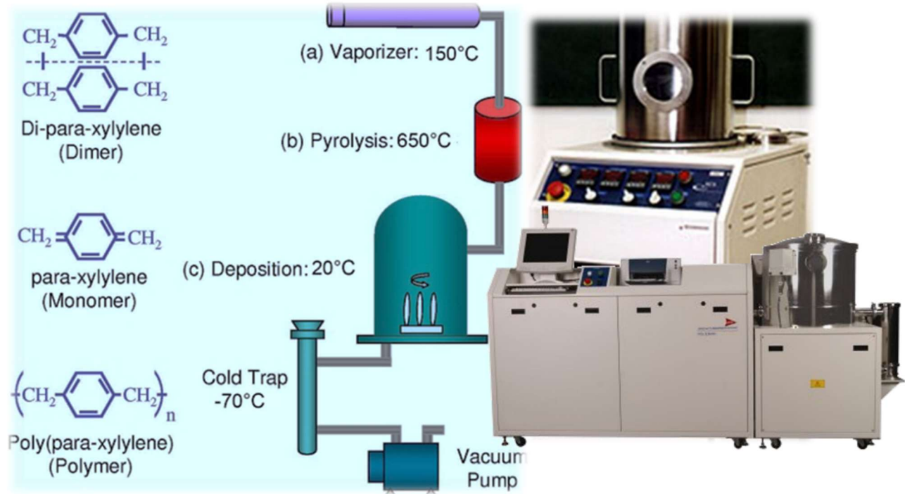
Figure 14: Parylene and the proposed ultra-thin oxide conformal coatings have to be deposited under stringent vacuum and temperature conditions. Not only raw material costs are substantially higher for Parylene, the application process cost and time are also limitations.
