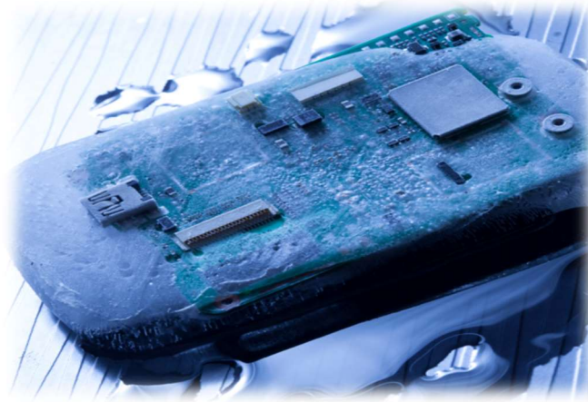
Figure 11: Representation of conformal coating protecting PWB with multiple components and solder joints. Besides having ability to prevent penetration to the PWB by moisture-water and harmful gases, the conformal coating must also withstand thermal cycling and thermal shock induced interfacial stress and stress concentration at corners and solder joints.
